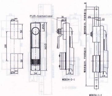
Dimensions of outline and cut out 外形及安装孔尺寸
