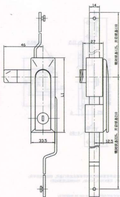
Dimensions of outline and cut out 外形及安裝孔尺寸
