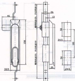
Dimensions of outline and cut out 外形及安装孔尺寸
