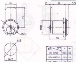
Dimensions of outline and cut out 外形及安装孔尺寸
