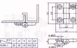
Dimensions of outline and cut out 外形及安装孔尺寸
