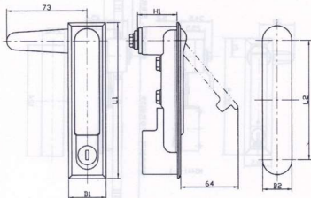
外形及安装孔尺寸 Dimensions of outline and cut out
