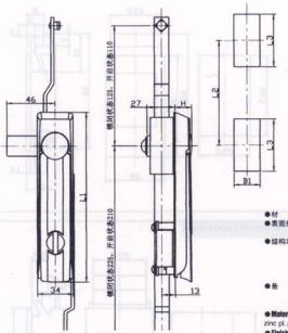
Dimensions of outline and cut out 外形及安裝孔尺寸
