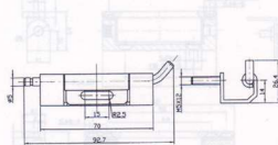
Dimensions of outline and cut out 外形及安装孔尺寸
