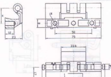
Dimensions of outline and cut out 外形及安装孔尺寸
