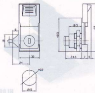
Dimensions of outline and cut-out 外形及安装孔尺寸
