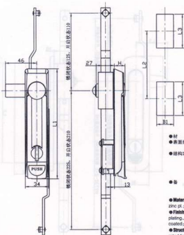
Dimensions of outline and cut out 外形及安裝孔尺寸
